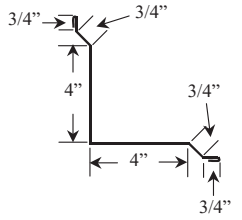
16. Inside Corner
