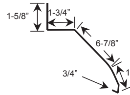
17. Cannonball Track Cover
