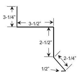
17. National Track Cover
