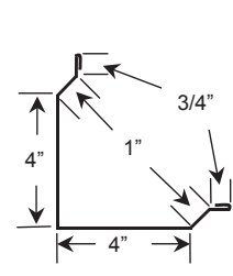
15. Outside Corner
