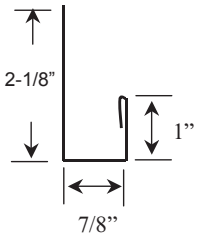
1. J Channel
