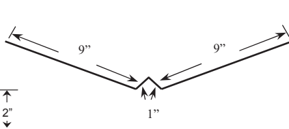
20. W Valley Trim
